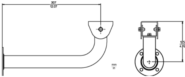
LTC 9212/00 Wall Mount, 300 mm (12 inch)
