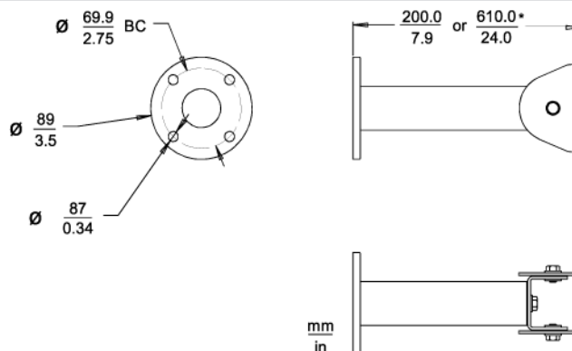
LTC 9210/00 Column Mount, 200 mm (8 inch) LTC 9223/00 Column Mount, 610 mm (24 inch)
